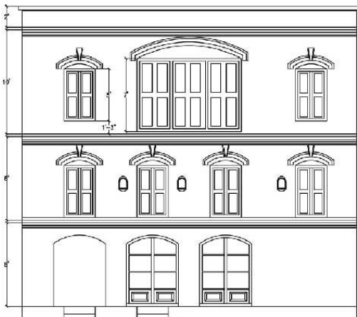
North Elevation
